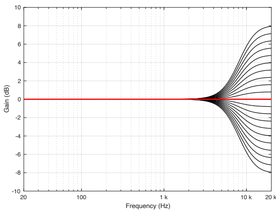
Figure 4.1: Frequency response measurements of all settings of the Treble control. Note that this response is applied to all input channels.
