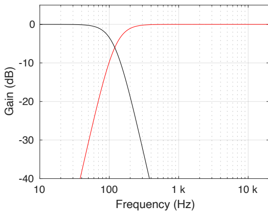
Figure 3.1: Gain response of the crossover used in the Bass Management system, showing an example with the factory-default crossover frequency of 120 Hz.
