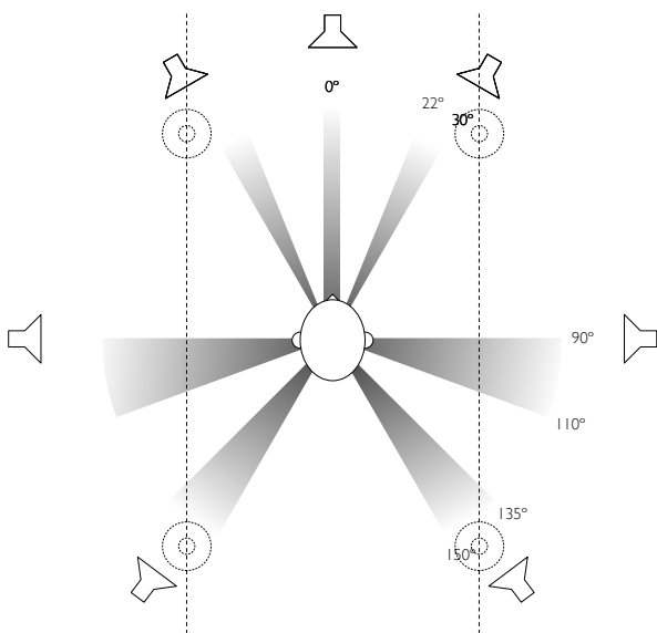
Figure 10.4: Loudspeaker positions associated with the speaker roles available in the Premiere, showing a full 7.x.4 configuration.
