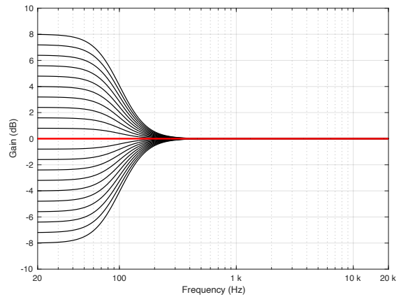
Figure 4.2: Frequency response measurements of all settings of the Bass control. Note that this response is applied to all input channels.
