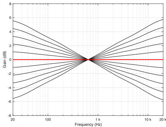
Figure 2.1: Frequency response measurements of all settings of the Frequency Tilt control. Note that this response is applied to all input channels.
