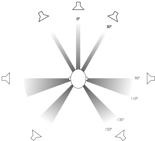
Figure 10.3: Recommended loudspeaker configuration for most 7.x channel audio signals. The actual angles of the loudspeakers shows the reference placement used at Bang & Olufsen for testing and tuning.
