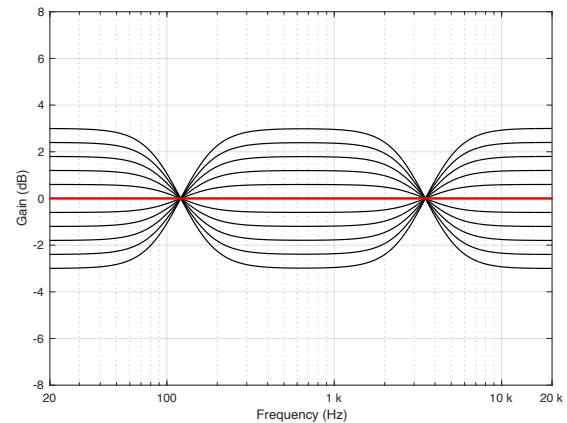
Figure 2.2: Frequency response measurements of all settings of the Sound Enhancement control. Note that this response is applied to all input channels.
